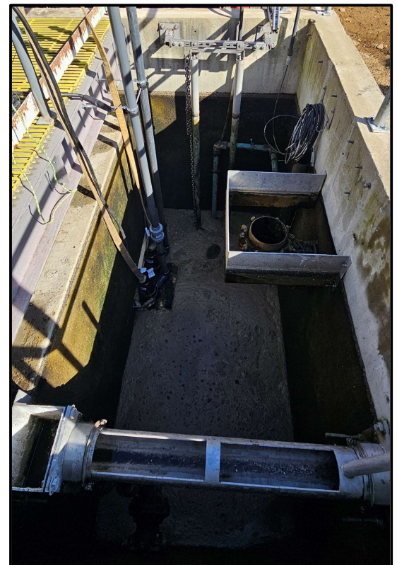
Setup of Temporary Bypass Pumping System in Existing Clearwell for Proposed Work on Final Effluent Piping
