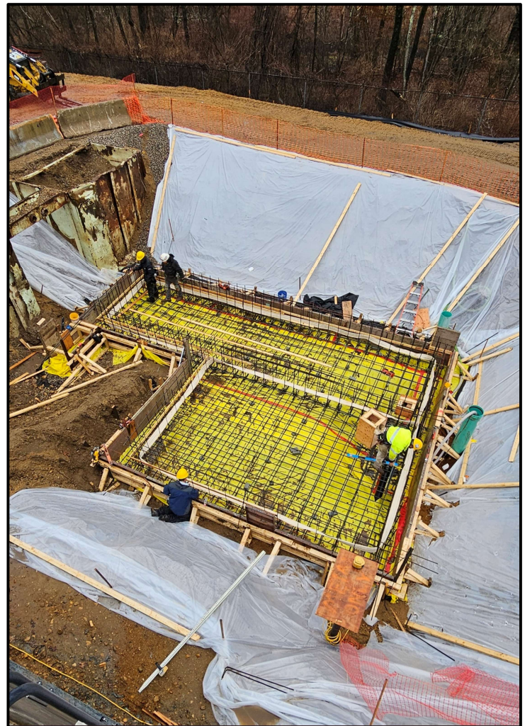
Installation of Forms and Rebar for New Effluent Building Slab
